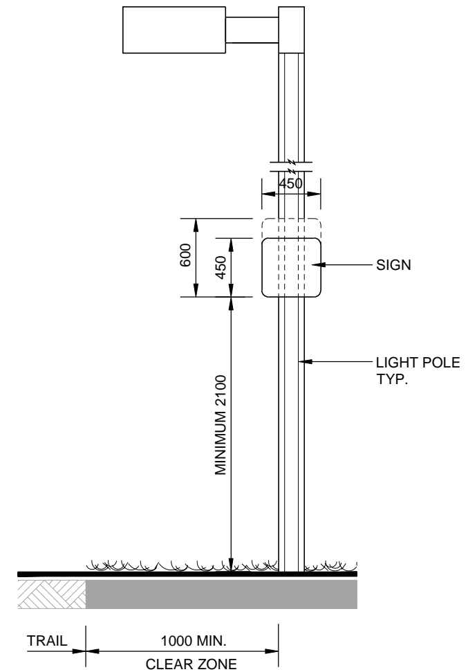
SIGN MOUNTED ON UTILITY POST
