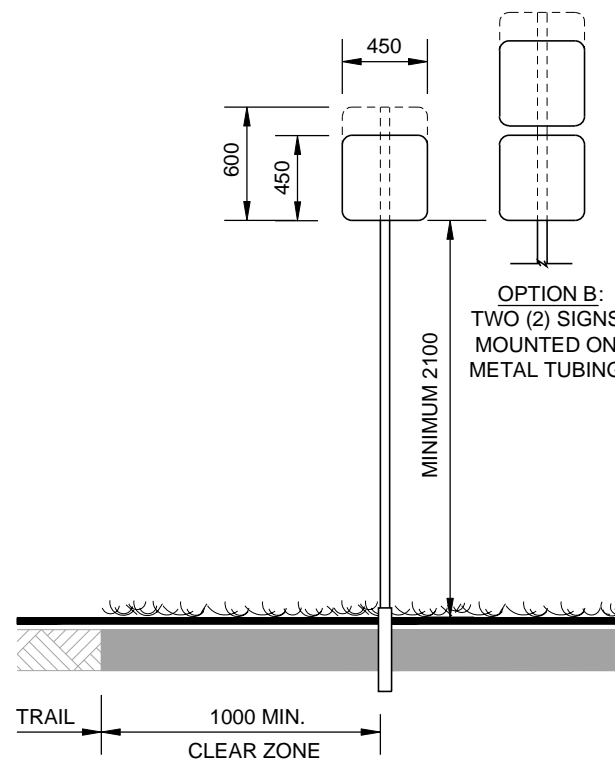
SIGN MOUNTED ON METAL TUBING
