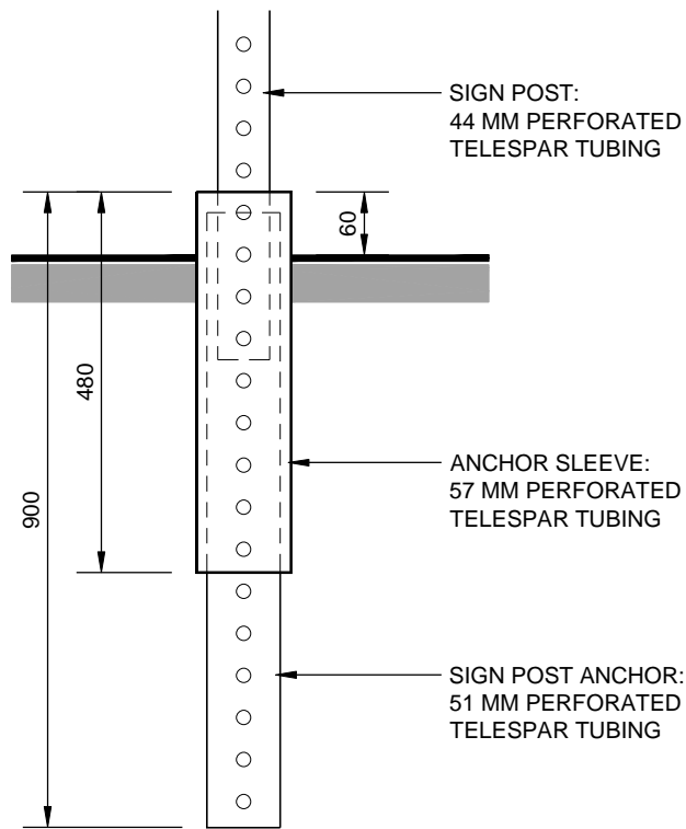
TUBING ANCHOR DETAIL
